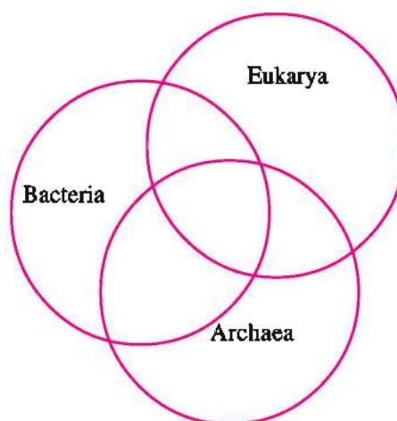
Three-domain classification
