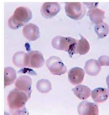
Plasmodium
