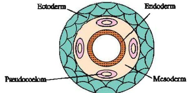
(B) Pseudocoelomate
