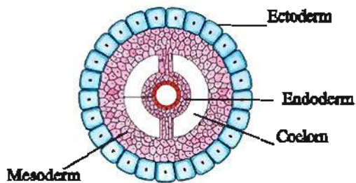
(A) Coelomate
