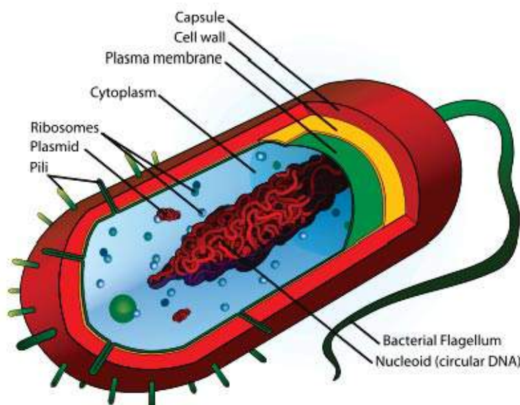
Prokaryotic cell
