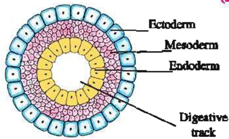
(C) Acoelomate
