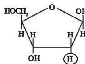
Deoxyribose Sugar
