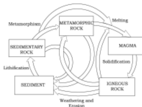
Fig 5.1 : Rock Cycle
