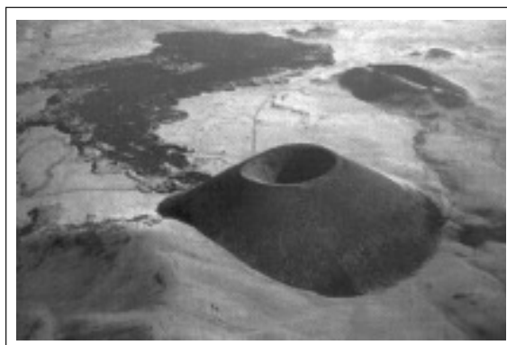
Shield Volcano
