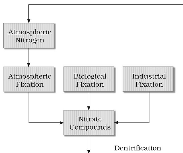
Figure 15.3 : Nitrogen Cycle
