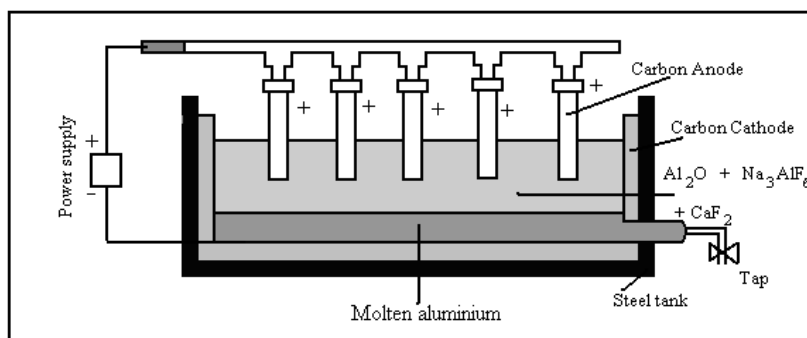
Electrolytic reduction of alumina
