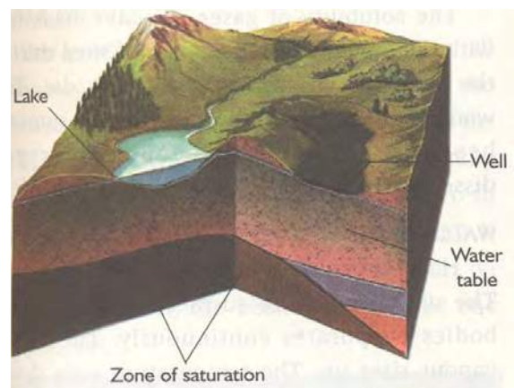
Fig.16.10: Ground water
