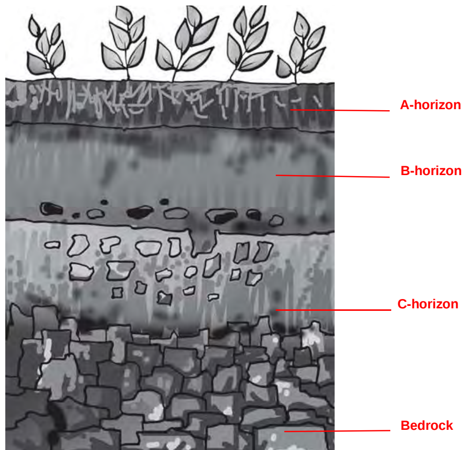
Fig.9.3 : Soil profile
