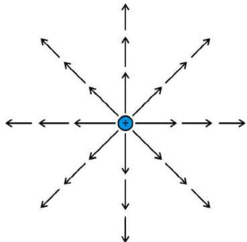
FIGURE 1.15 Field of a point charge.
