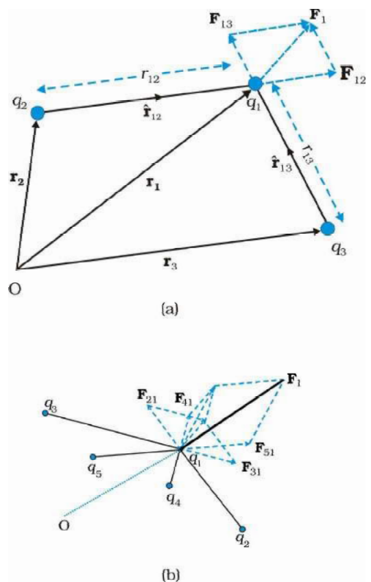
FIGURE 1.8 A system of (a) three charges (b) multiple charges.
