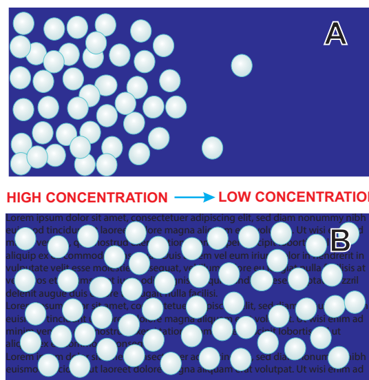
Figure 11.2: Distribution of molecules in diffusion (A) Initial stage (B) Final stage
