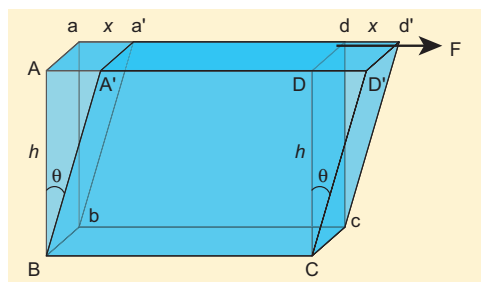
Figure 7.6 Shearing strain
