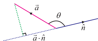
Negative dot product
