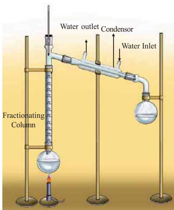
Fig. 4.8 Fractional Distillation
