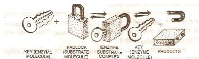
Mechanism of Enzyme Action : Lock and Key Model
