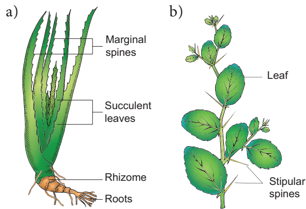
Figure 6.21: a) Succulent xerophyte – Aloe b) Non succulent perennial - Zizyphus
