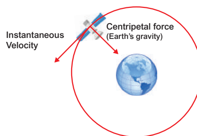
Figure 9.5 Orbital velocity
