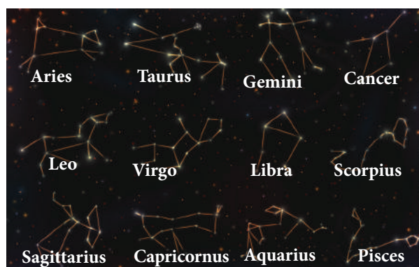
Figure 9.3 Constellations
