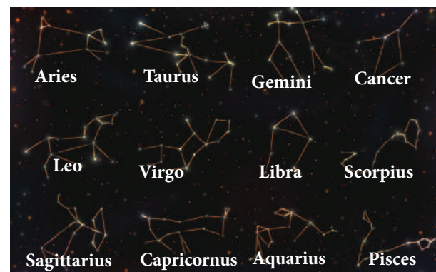
Figure 9.3 Constellations
