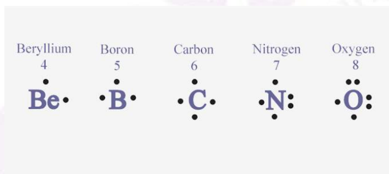
Lewis structures of elements with atomic number 5-8
