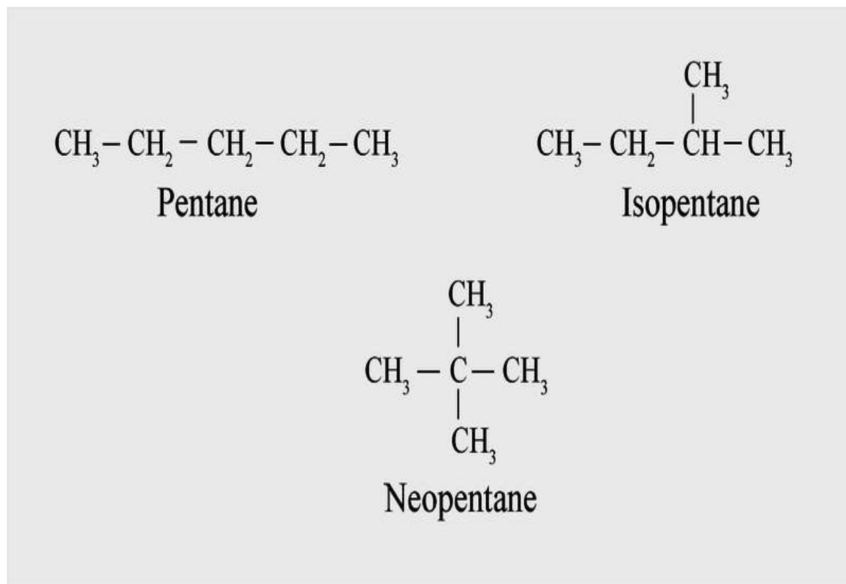
Structural isomers with molecular formula - C 5 H 12
