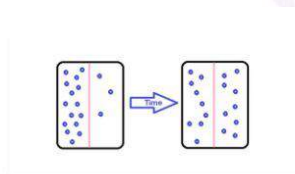
Diffusion of gas molecules
