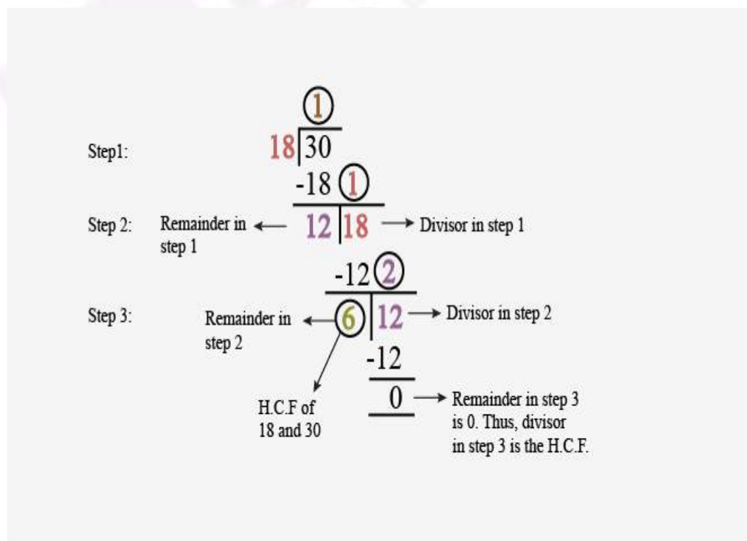
Finding the HCF of 18 and 30
