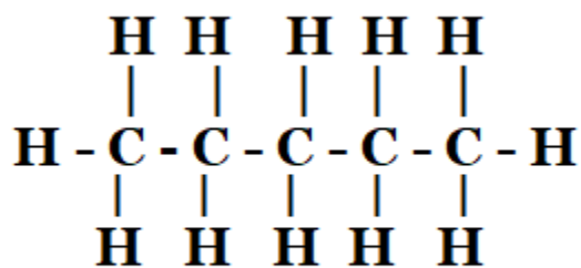
n-pentane
