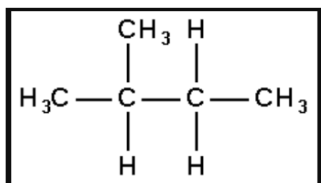
2-methylbutane
