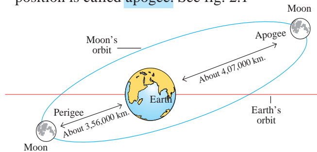
Figure 2.1 : Moon's positions
