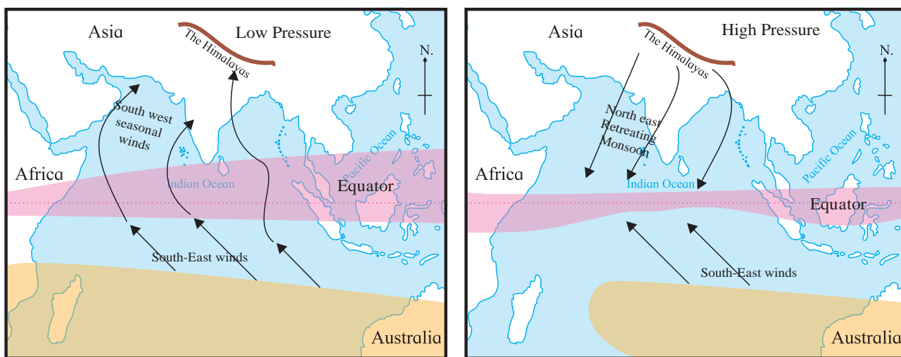
Figure 5.6 : Seasonal winds
