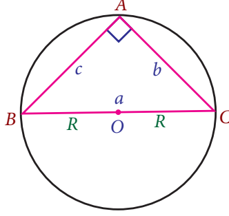
\angle A = 90^\circ
