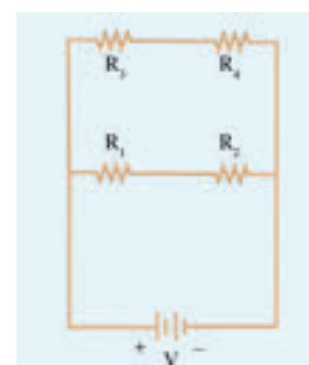
Figure 4.9 Parallel-series combination of resistors
