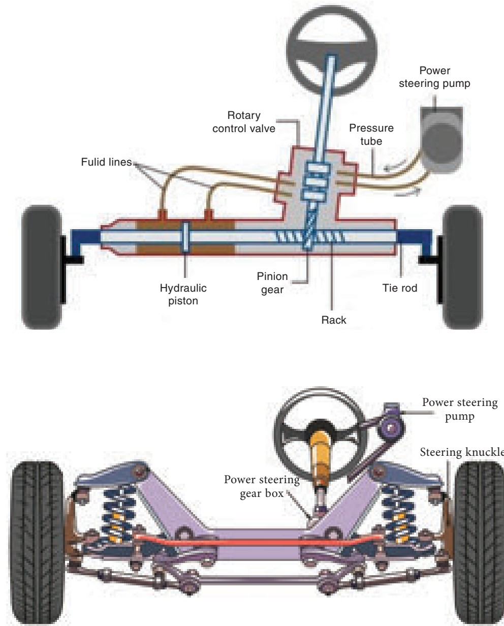
Figure 8.4 Power steering
