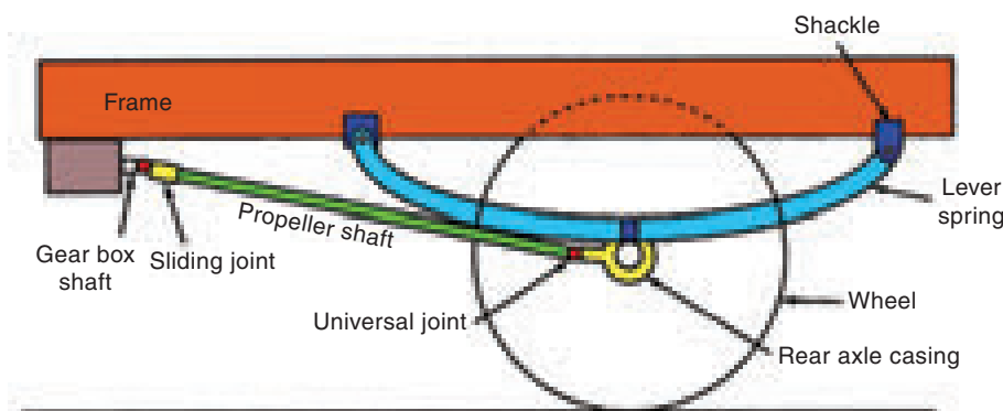
Figure 4.3.1 Hotchkiss drive
