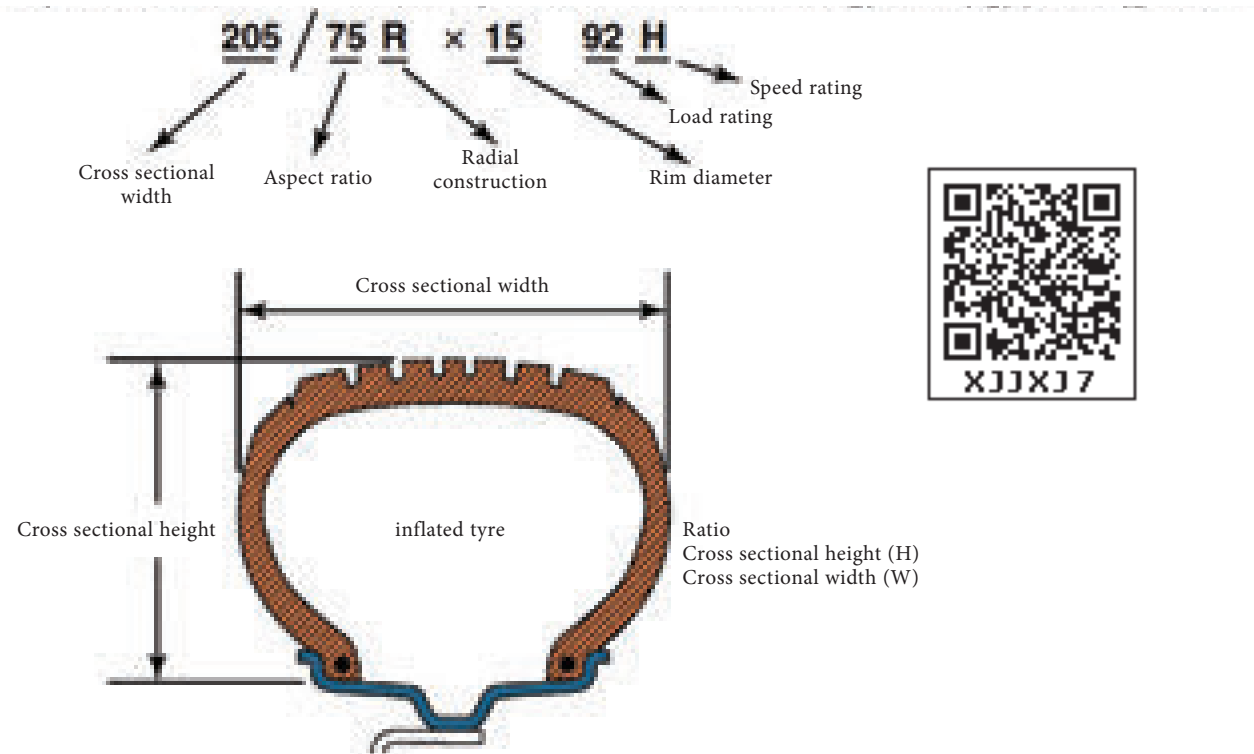
Figure 5.10.1 The tyre specifications.
