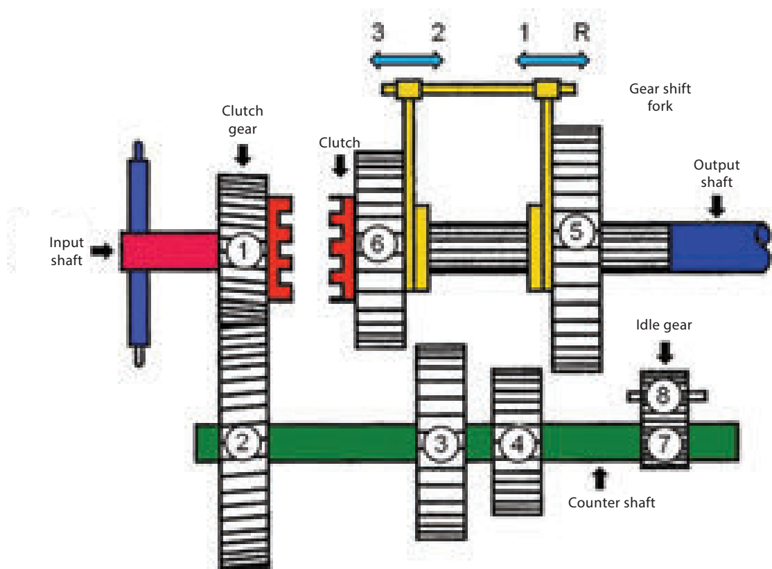
Figure 3.5.1 Sliding mesh gear box
