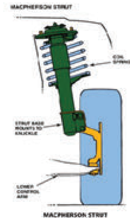
Figure 7.3.2.4 MacPherson Strut types
