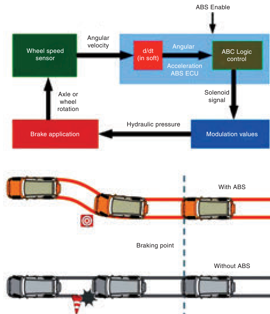
Figure 6.6 Effect of ABS on the Vehicle
