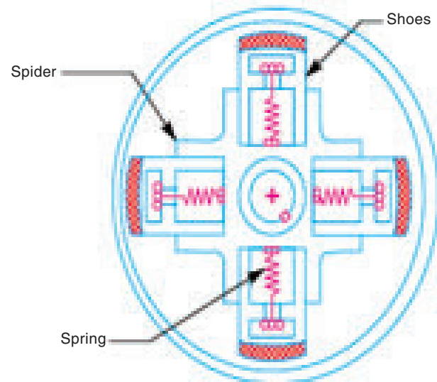
Figure 2.5.5 (a) Centrifugal clutch
