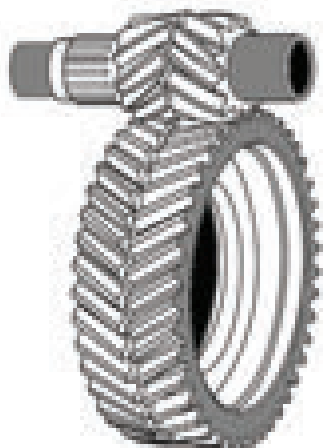
Figure 3.2.1.6 Double helical gear of herringbone gear
