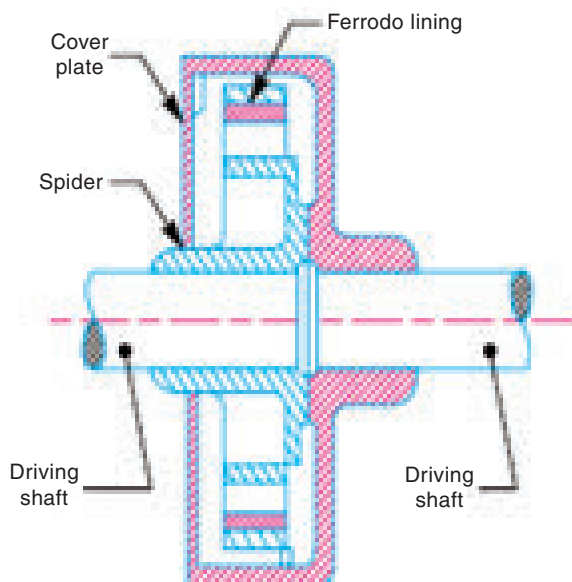
Figure 2.5.5 (a) Centrifugal clutch
