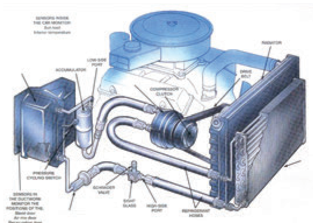
Figure 10.12.1 (a) Air conditioning System
