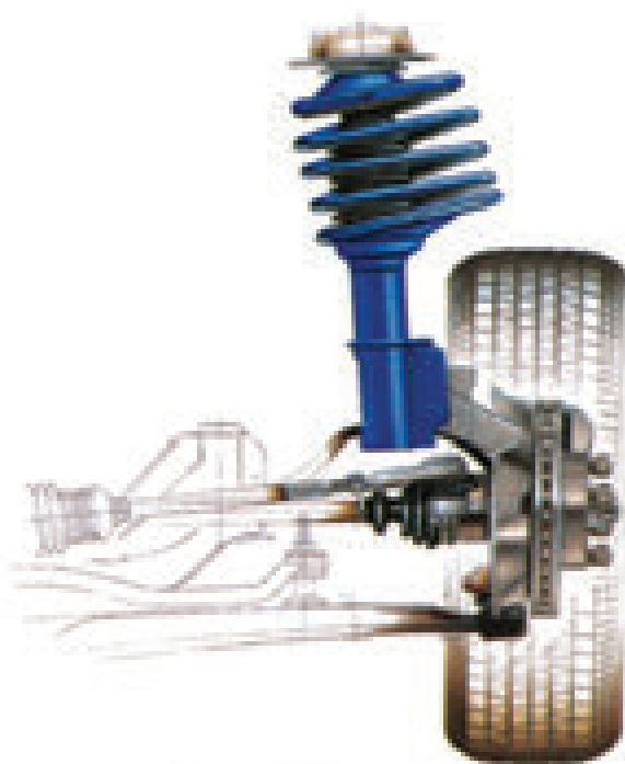
A front MacPherson strut assembly.
