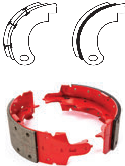
Figure 6.8.2 Brake shoes
