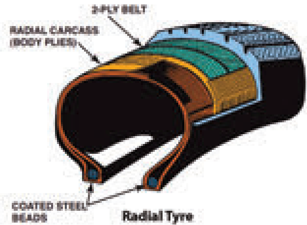
Figure 5.11.1 View of a radial ply tyre
