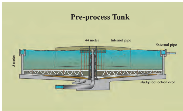
Sedimentation Tank
