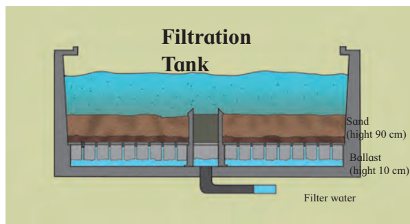
Filtration Tank
