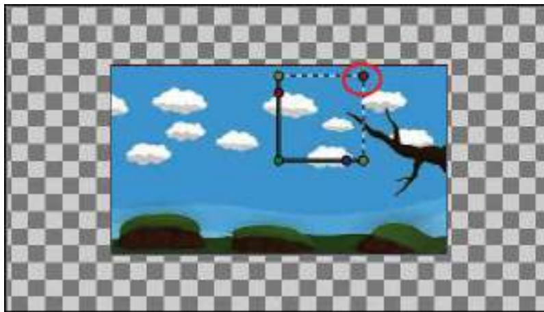
Fig. 9.14 Selection Handles
